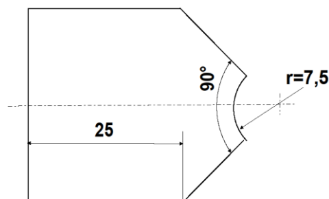
TEMPLATE FOR NOSE-/SPINNER-RADIUS
